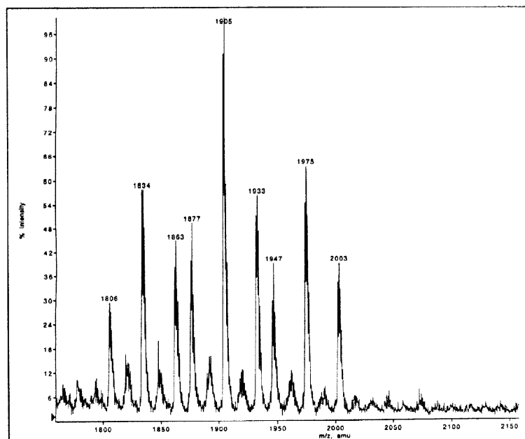
Figure 3. ESMS of the tetramer homodimer sublibrary (9) derived from A1B13C1–C4 (10 components with 9 different molecular weights)
